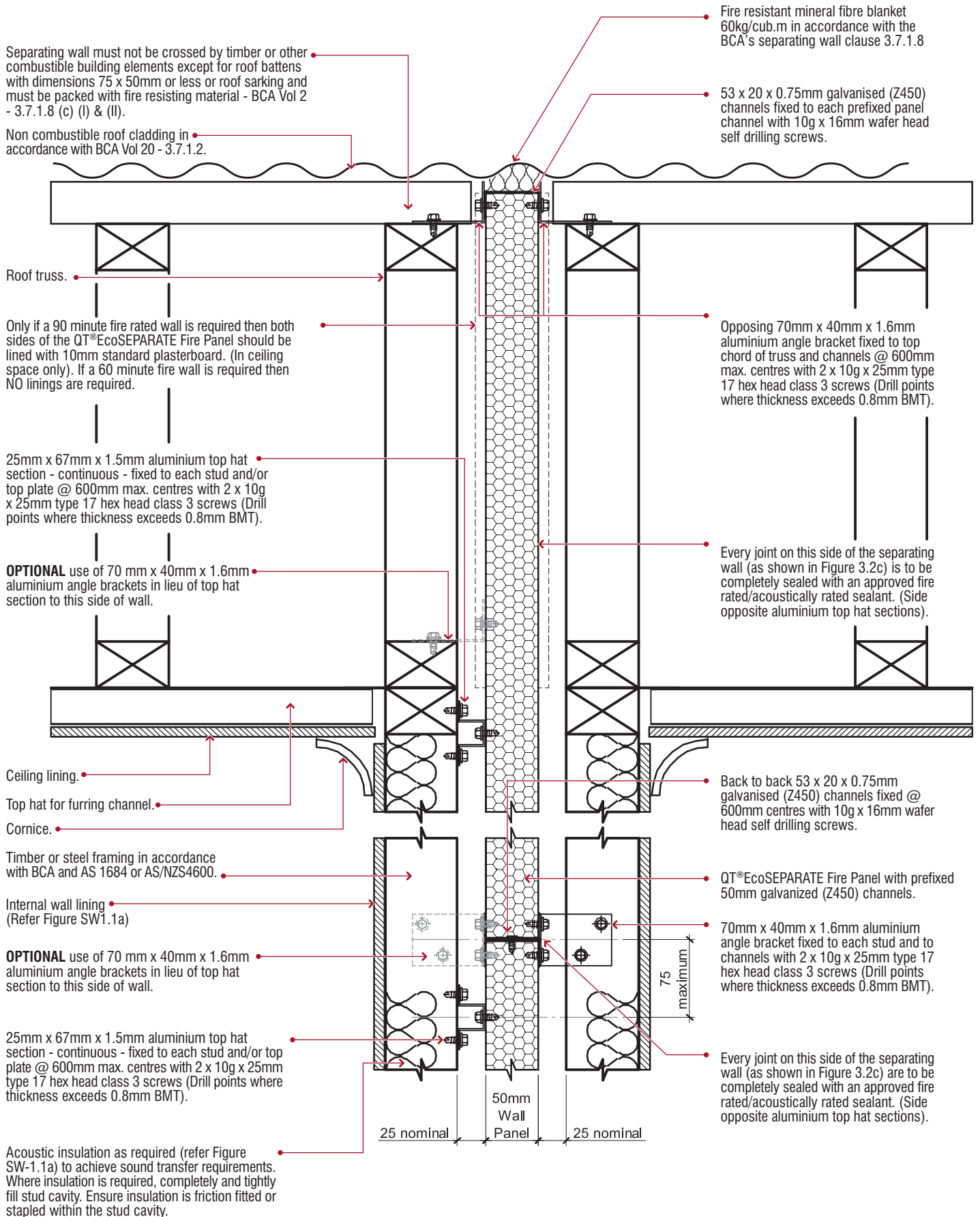
Figure 2.3 (c) - Truss Zone
